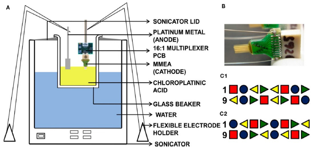
Figure 2.1 The sonicplating setup and microelectrode array.
